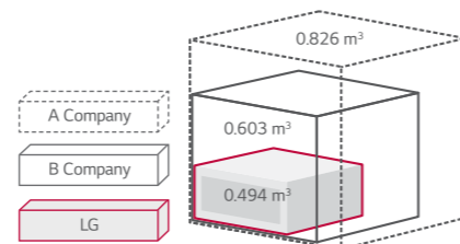
Volume (Heat Exchanger Module)
